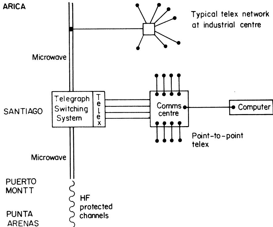
Figure 2. Nature of Telecommunications using existing public system. This cannot yet accept even low speed data. System uses Alphabet No. 2 at 50 Bauds.
